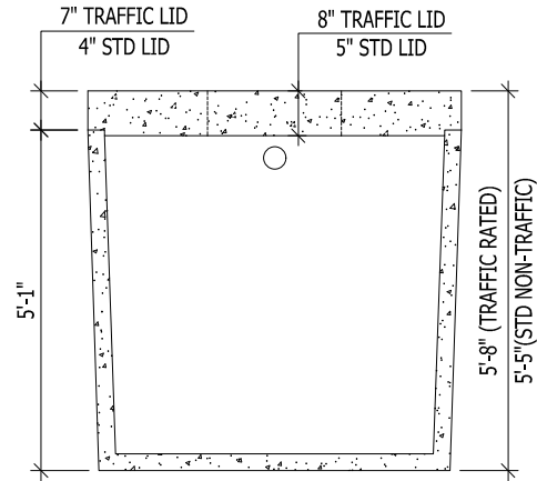
SECTION B
