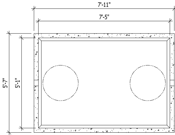
PLAN SECTION
