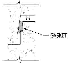
GASKET DETAIL SCALE: NTS
