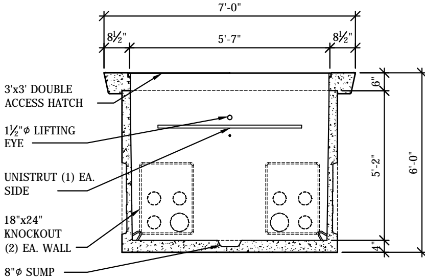
SECTION A
