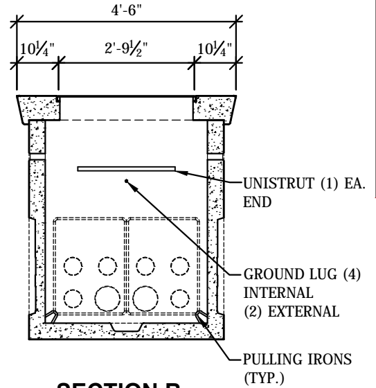
SECTION B
