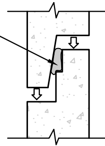
DETAIL A
