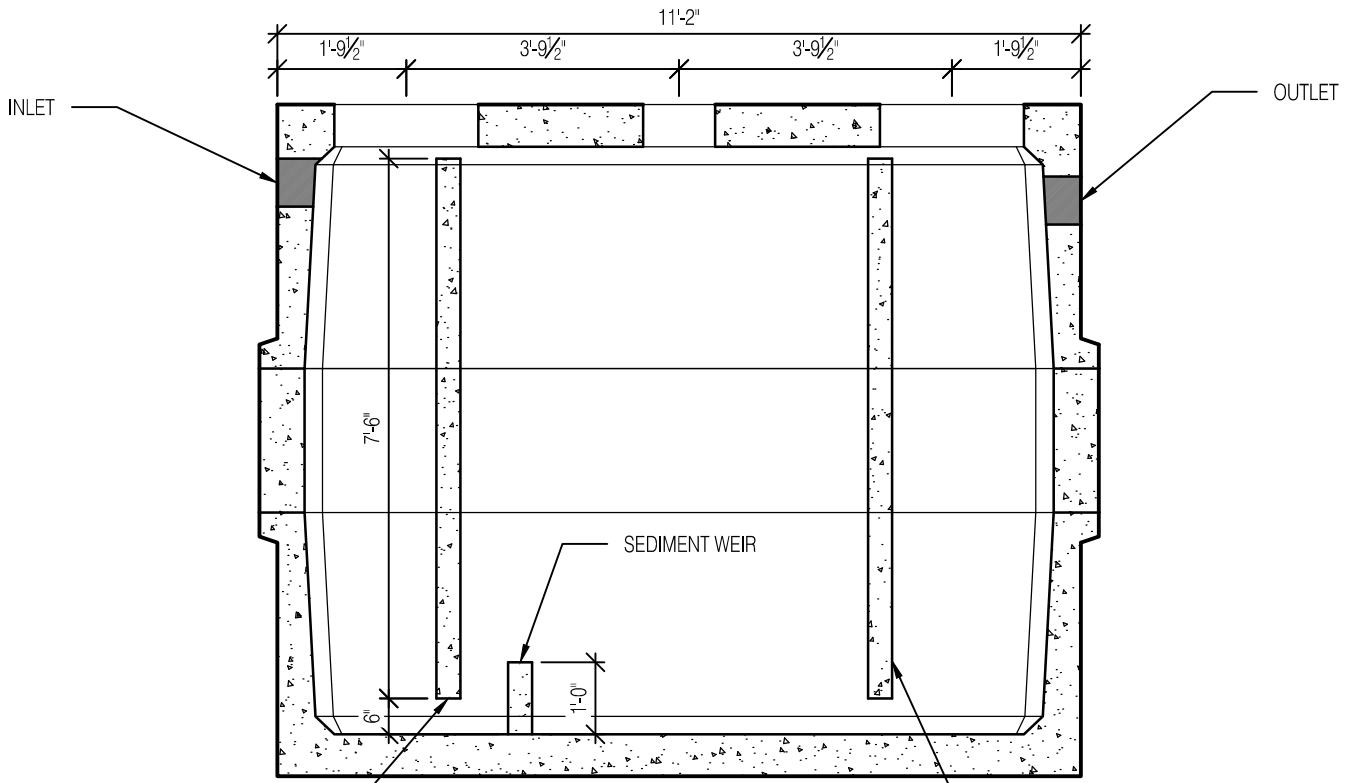
(A) SECTION
