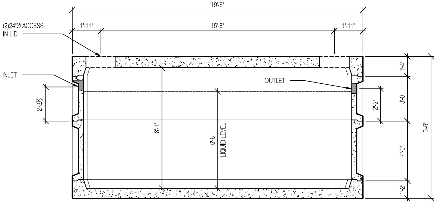
A SECTION
